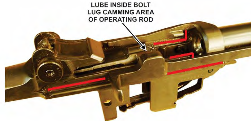
Figure 66. Lubrication
