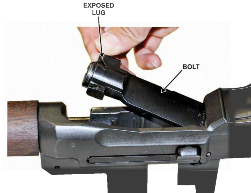
Figure 23. Bolt removal by exposed lug
