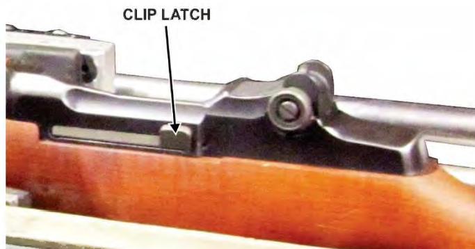
Figure 2. Clip latch
