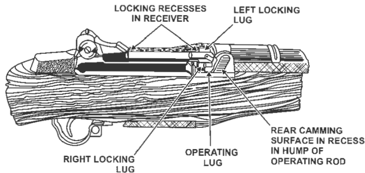
Figure 60. Locking
