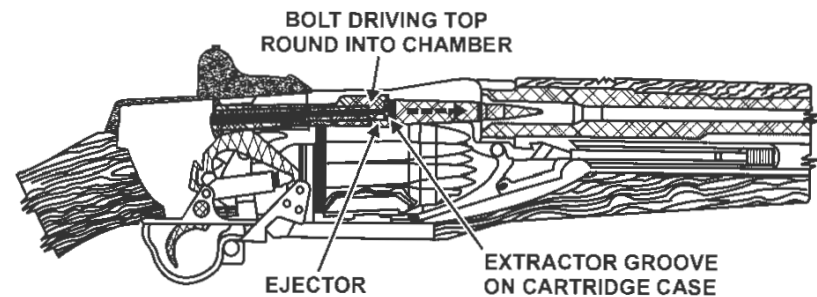
Figure 59. Chambering
