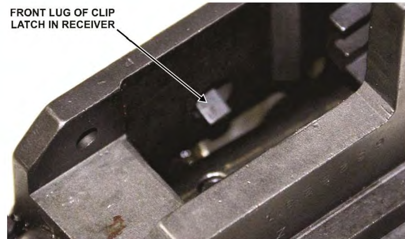
Figure 44. Lug in receiver
